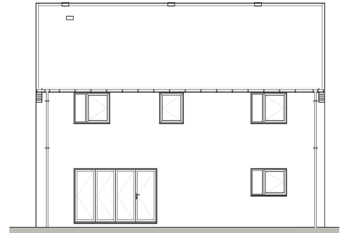
REAR ELEVATION
